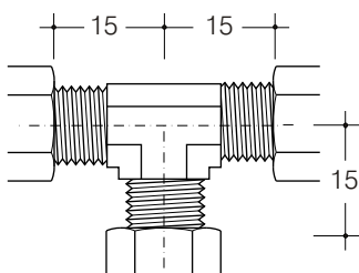
Modello / Model: AR270T
