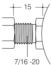
Modello / Model: AR000
