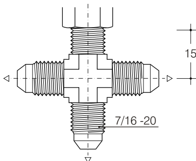
Modello / Model: AR360T
