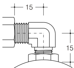
Modello / Model: AR090
