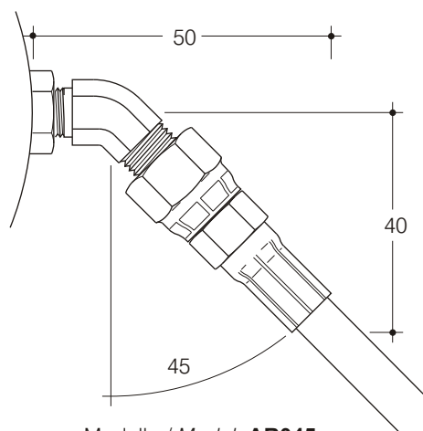
Modello / Model: AR045
