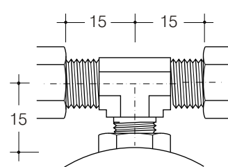
Modello / Model: AR270
